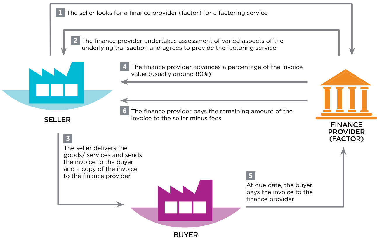
Figure 7: Factoring
